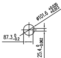
Shaft Dimension
