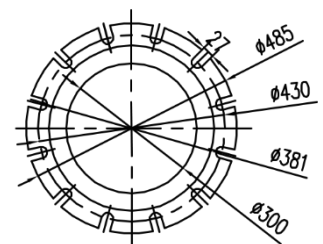
Suction Flange
